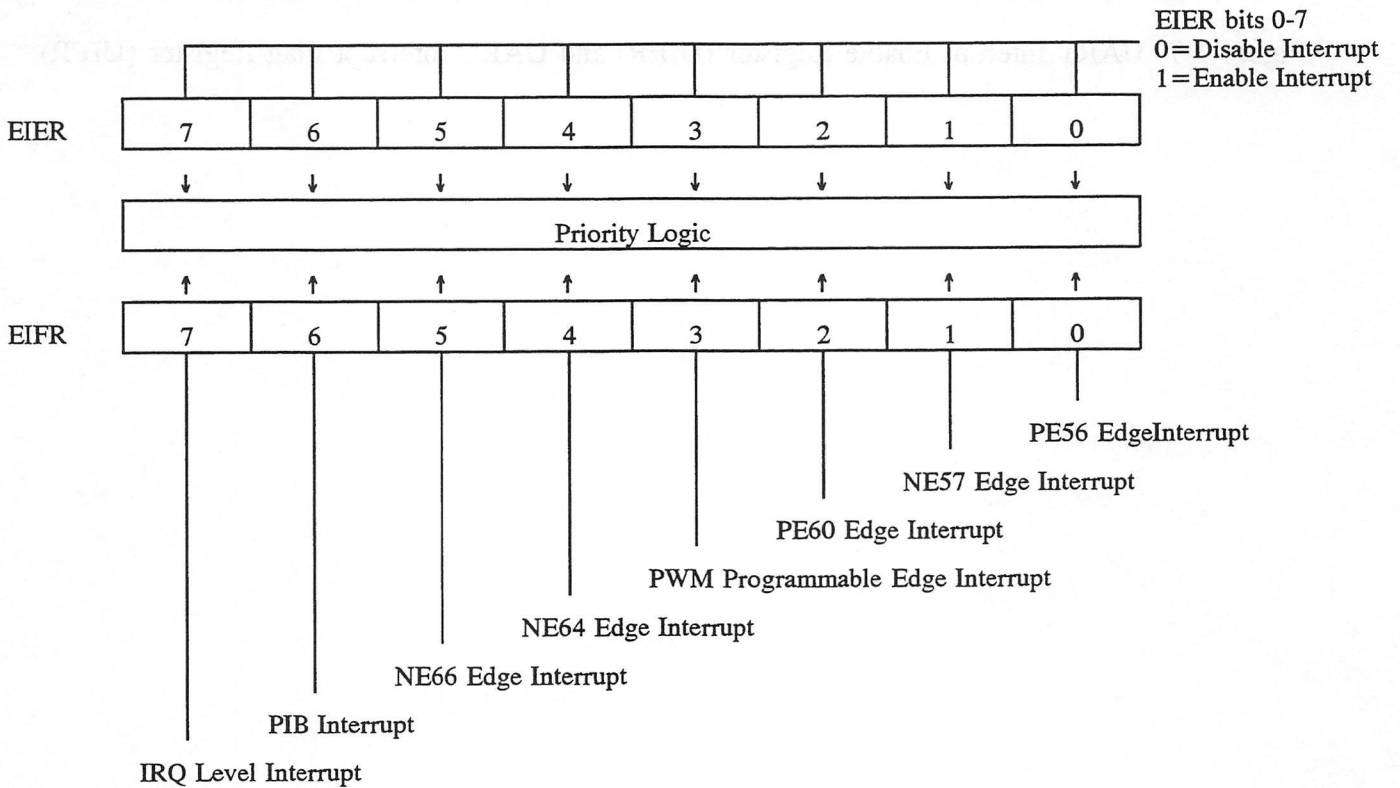
Figure 1-6 Edge Interrupt Enable Register (EIER) and Edge Interrupt Flag Register (EIFR)
