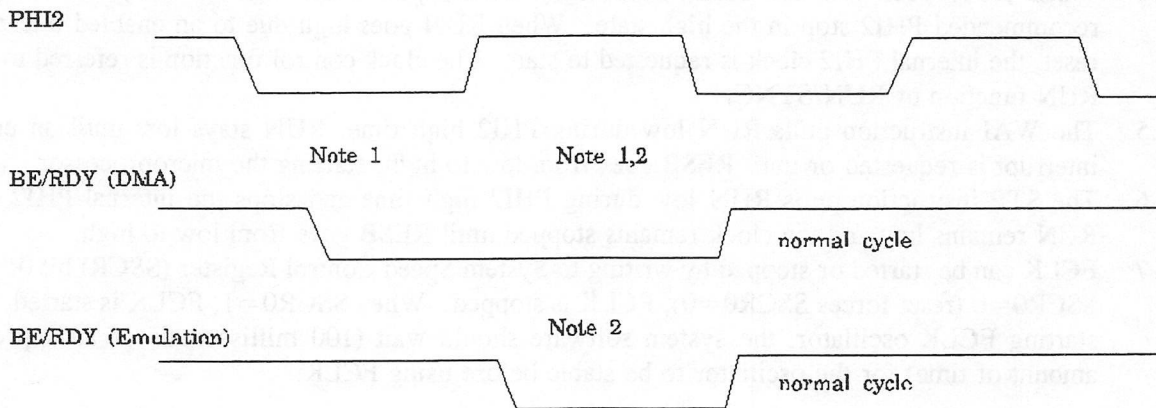
Figure 2-5 BE/RDY Timing Relative to PHI2
