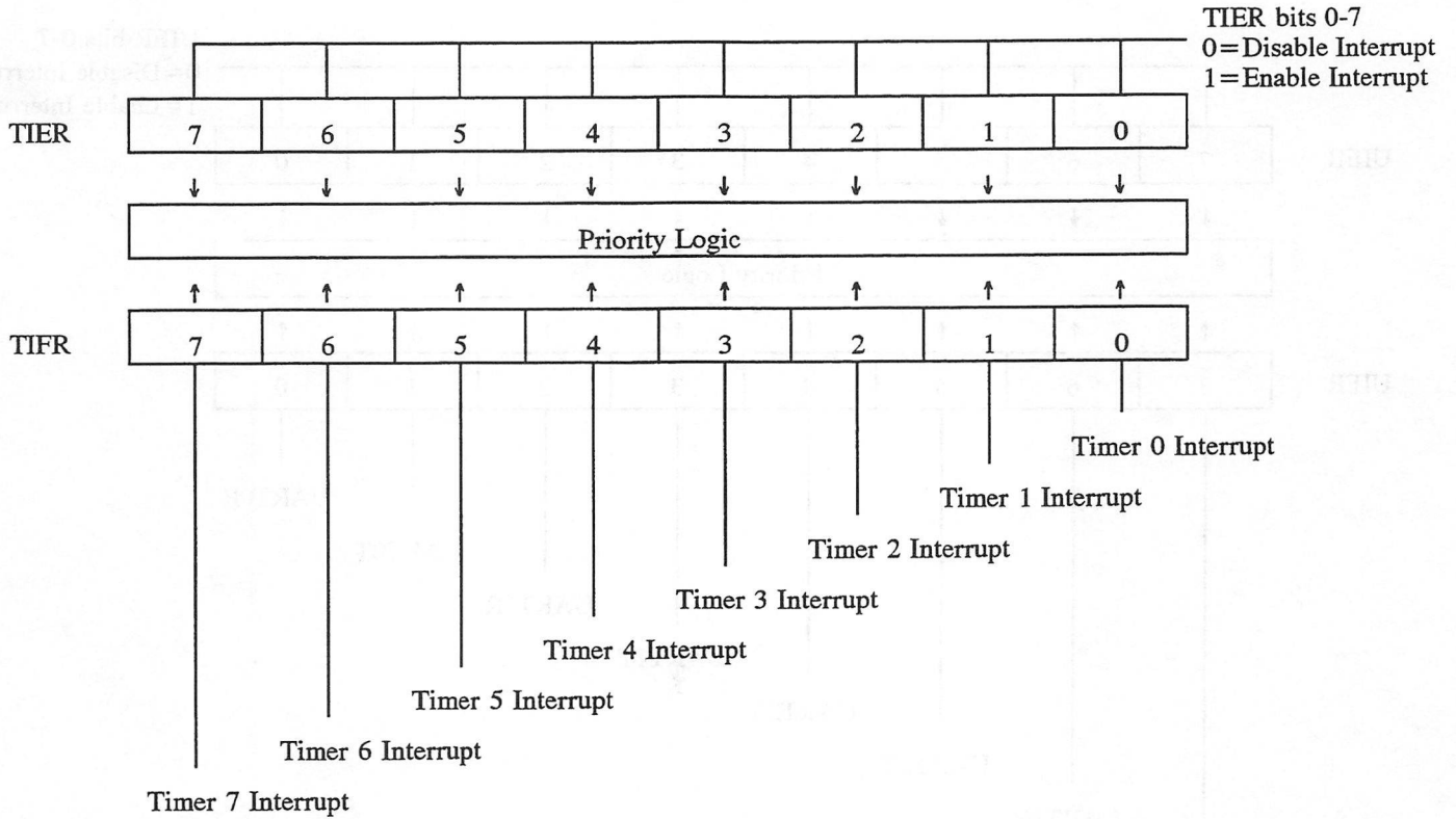
Figure 1-5 Timer Interrupt Enable Register (TIER) and Timer Interrupt Flag Register (TIFR)
