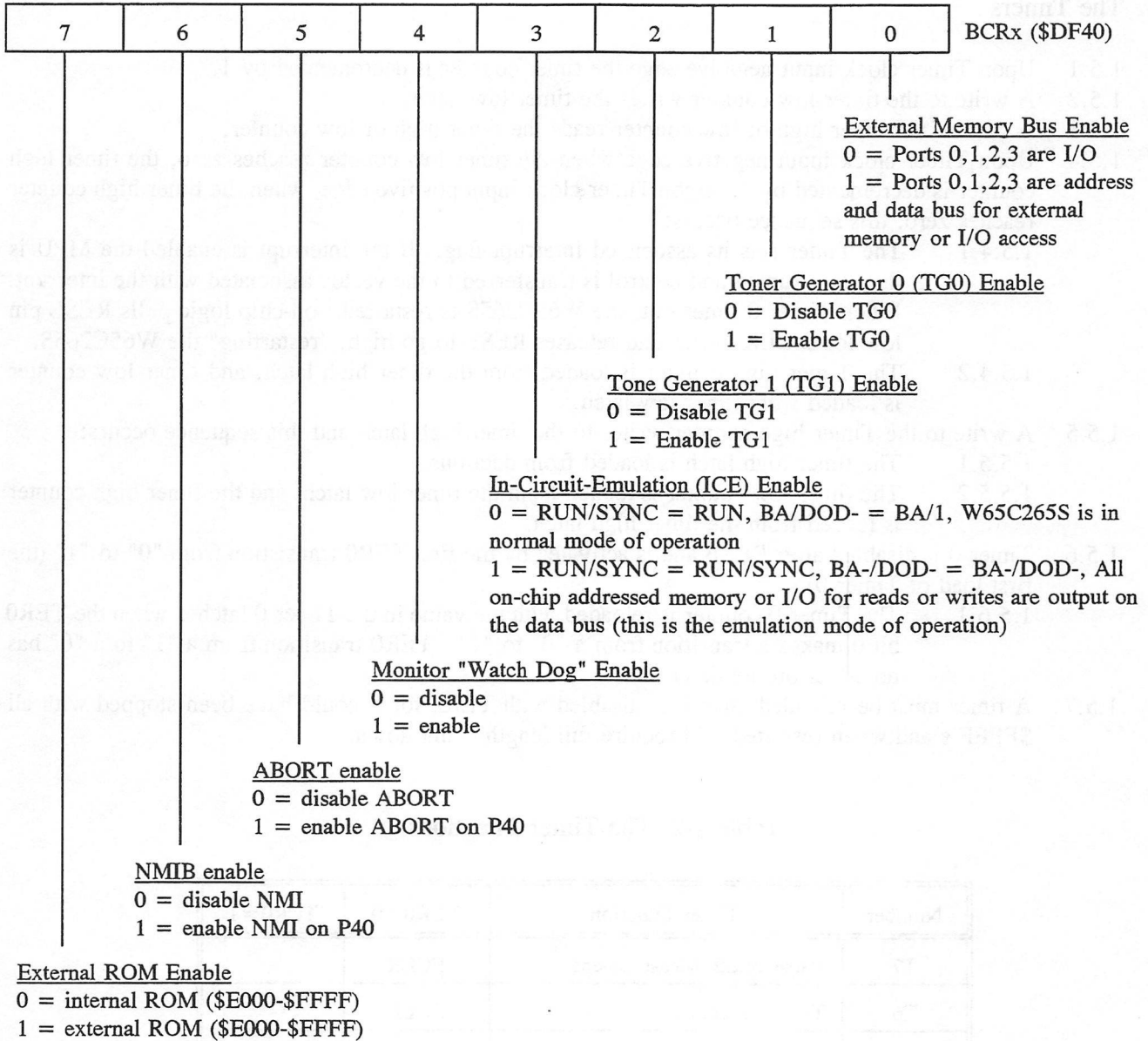
Figure 1-2 Bus Control Register (BCR)
