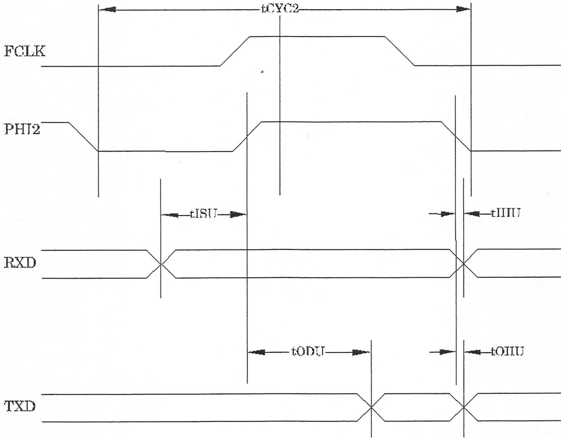
Figure 3-4 AC Timing Diagram #4
