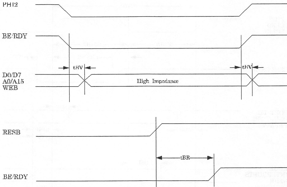
Figure 3-3 AC Timing Diagram #3
