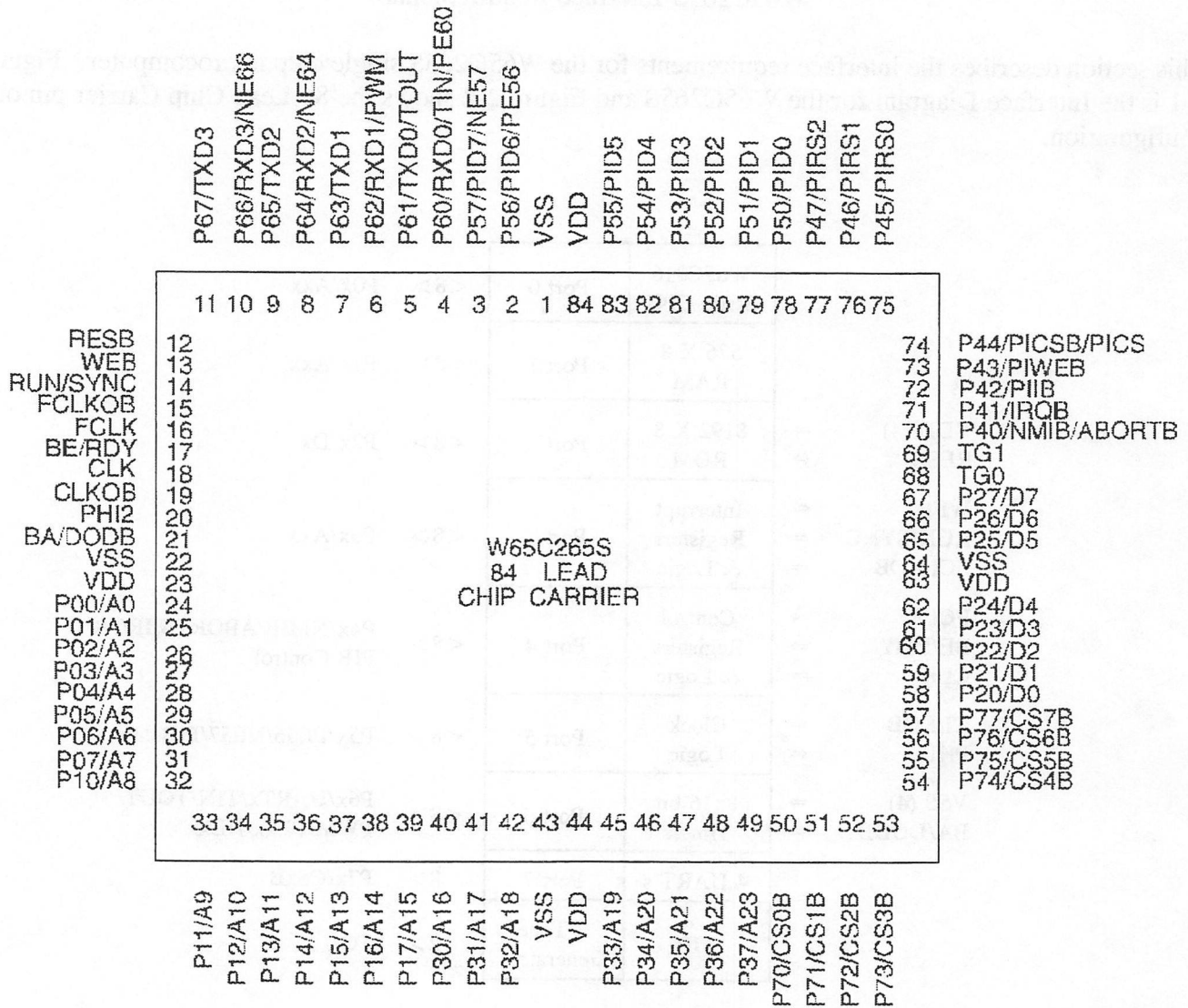
Figure 2-2 W65C265S 84 Lead Chip Carrier Pinout Designation
