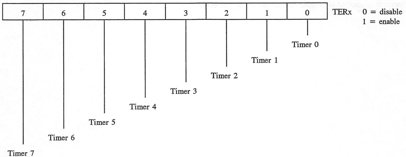
Figure 1-4 Timer Enable Register (TER)
