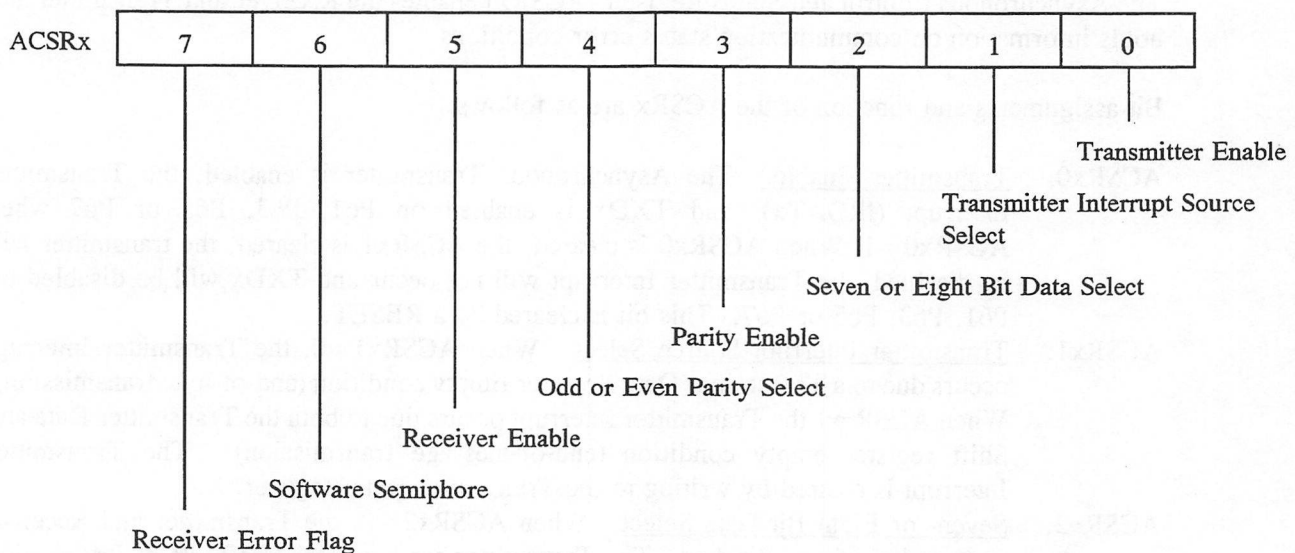
Figure 1-10 ACSRx Bit Assignments
